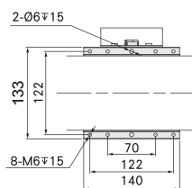
B-Detail View
