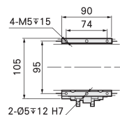
B-Detail View
